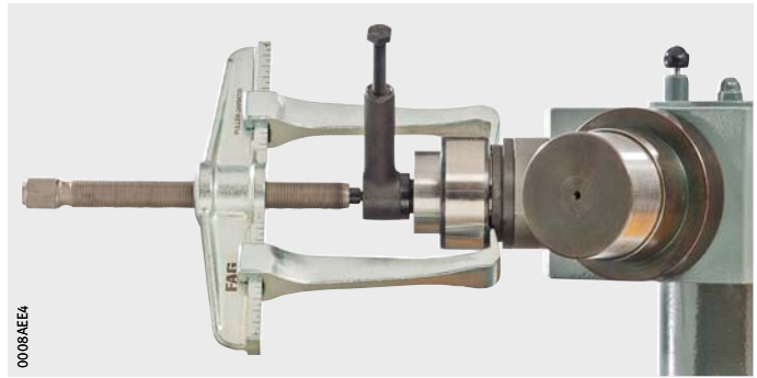
Figure 7 Two-arm extractor with hydraulic pressure tool
