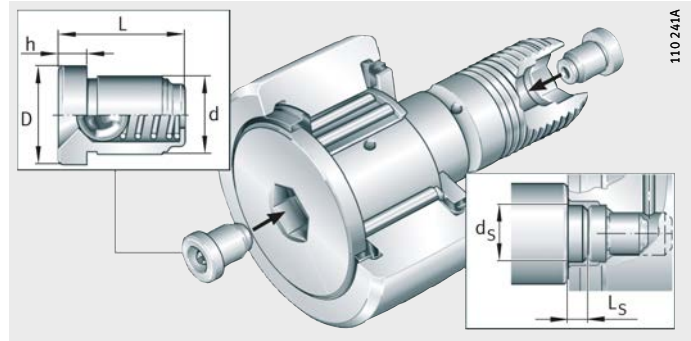
Figure 21 Stud type track roller with drive fit lubrication nipple and dimensions for pressing mandrel
