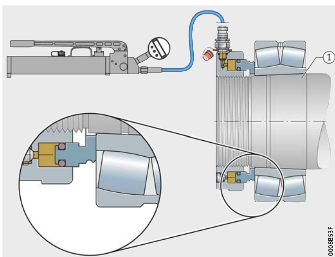
Figure 19 Mounting of a spherical roller bearing using a hydraulic nut
