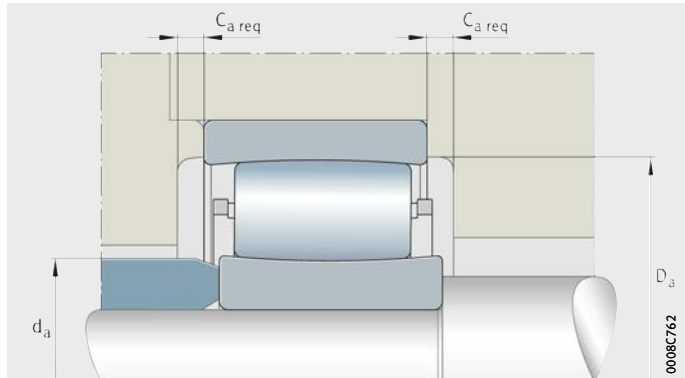
Figure 7 Free spaces in the housing
