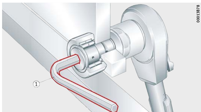
Figure 22 Holding the bearing using an Allen key
