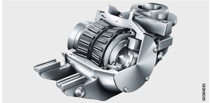
Figure 8 Wheelset bearing for rail vehicles
