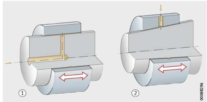
Figure 21 Principle of hydraulic mounting: creation of a fluid film between the fit surfaces
