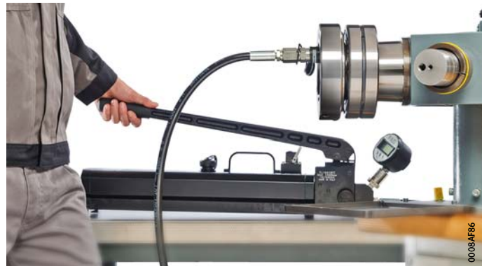
Figure 14 Hydraulic dismounting of tapered seat
