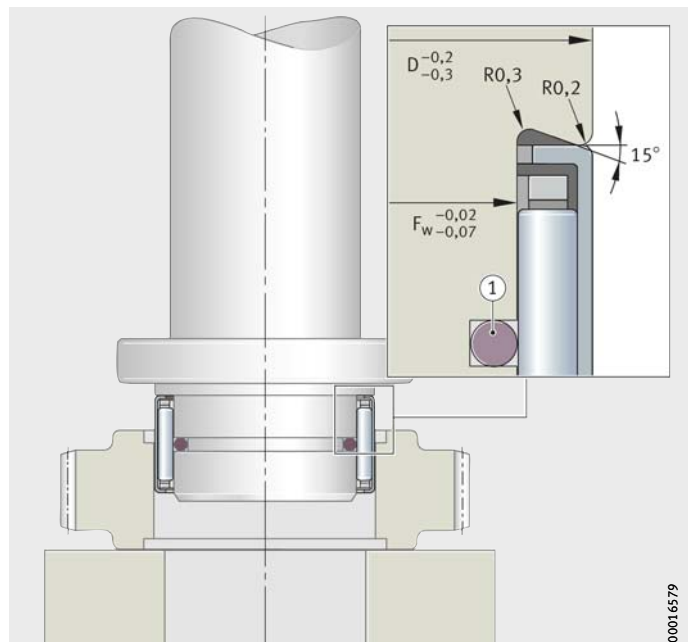
Figure 14 Mounting using pressing mandrel
