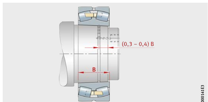
Figure 22 Recommended width for oil grooves
