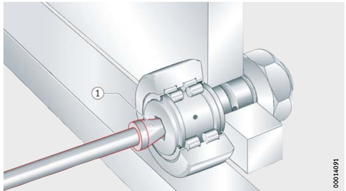
Figure 23 Relubrication using grease gun
