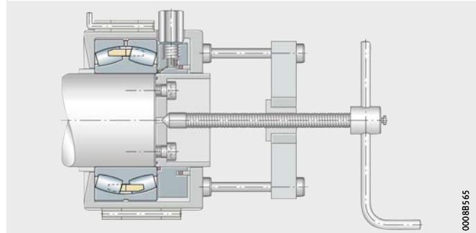
Figure 13 Special device for extraction from a shaft without oil grooves
