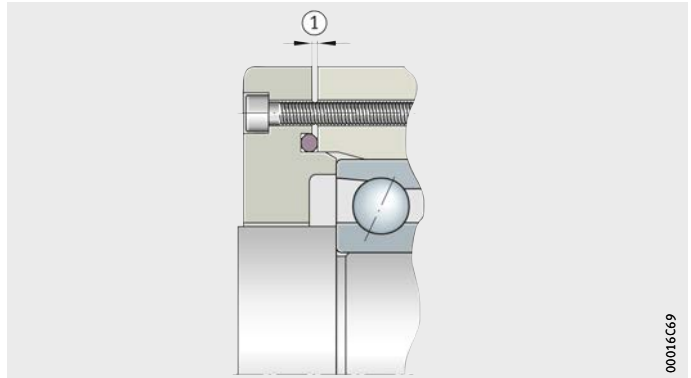
Figure 6 Matching of end cover (recommendation)
