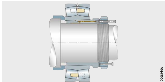
Figure 24 Bearing seat on the withdrawal sleeve
