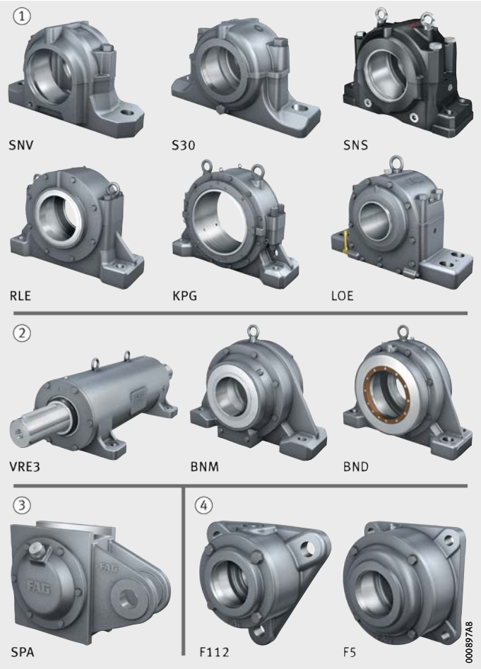
Figure 1 Bearing housings
