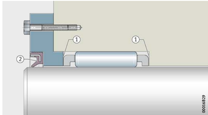
Figure 15 Guidance of needle roller and cage assemblies
