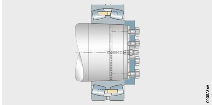
Figure 23 Bearing seat on the shaft
