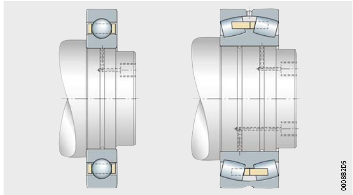
Figure 12 Hydraulic dismounting of cylindrical seat
