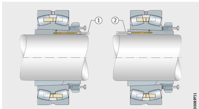
Figure 25 Bearing seat on the adapter sleeve
