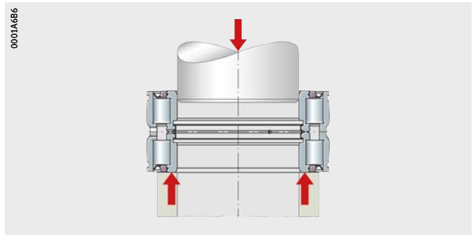
Figure 16 Application of mounting forces
