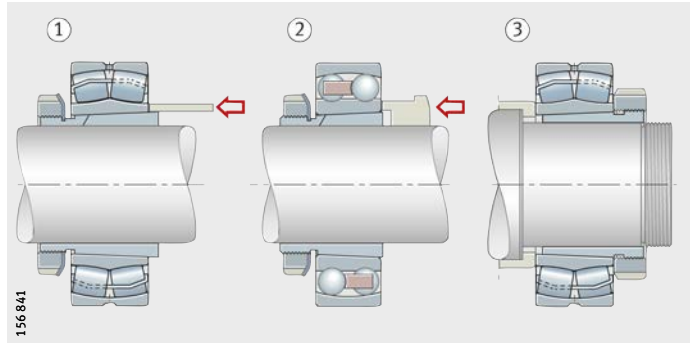
Figure 8 Dismounting of bearings
