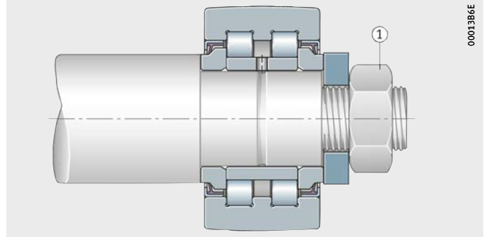
Figure 20 Axial location
