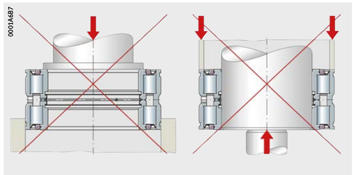
Figure 17 Impermissible mounting or dismounting methods
