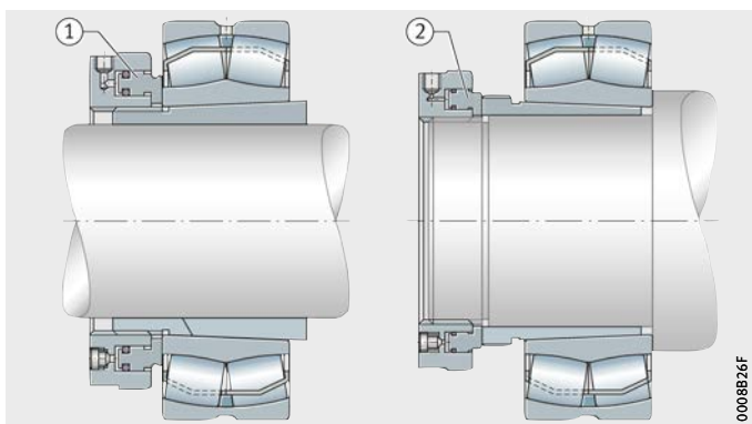
Figure 20 Mounting of a spherical roller bearing using a hydraulic nut
