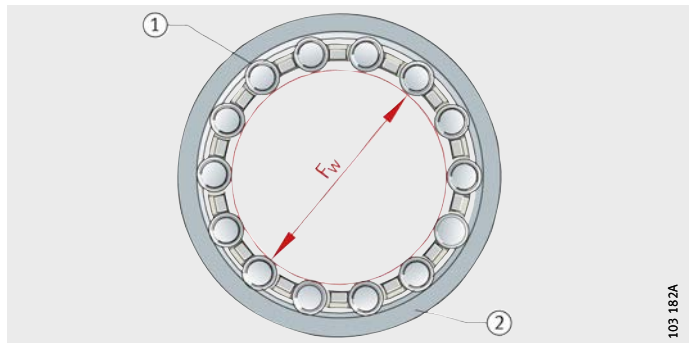
Figure 4 Enveloping circle
