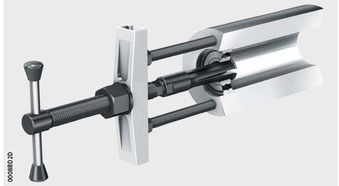
Figure 6 Internal extractor
