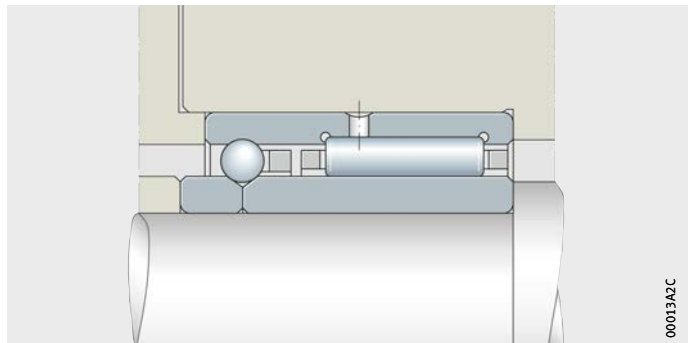
Figure 13 Mounting of combined needle roller bearings (needle roller/ angular contact ball bearing)
