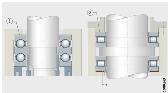
Figure 5 Axial bearings adjusted free from clearance
