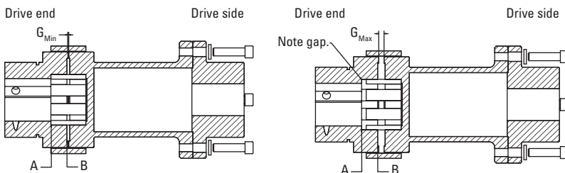
Fig. 2. Proper shaft-to-hub engagement.
