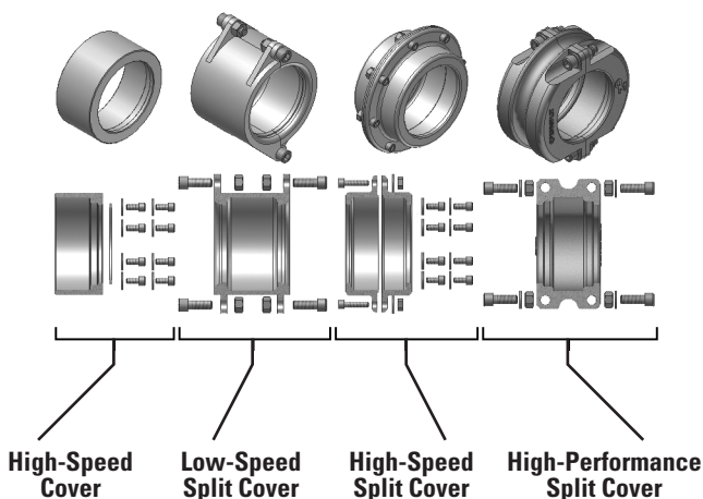
Fig. 1. Quick-Flex cover types and included hardware.
